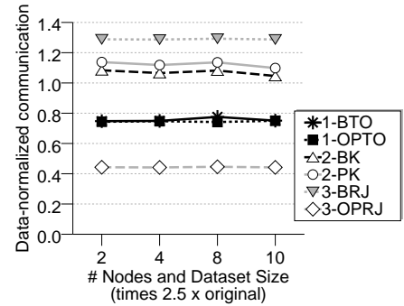
Figure 18: Data-normalized communication in each stage for self-joining the DBLP \times n dataset ( n \in [5, 25] ) increased proportionally with the increase of the cluster size.
